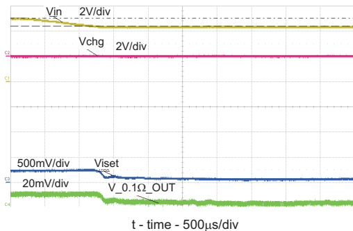
CH4: Iout (0.2A/Div) Figure 14. ISET Shorted Prior to USB Power-up
