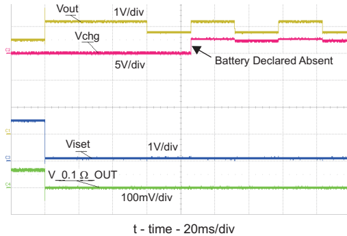
Figure 11. Battery Removal with fixed TS = 0.5V
