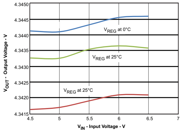
Figure 23. Line Regulation
